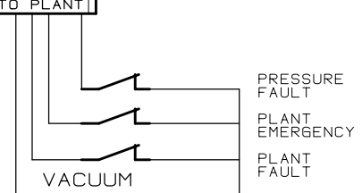
CONTACTS & PRESSURE SWITCHES
