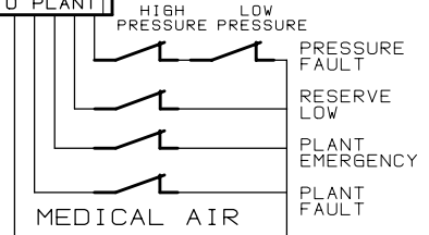
CONTACTS & PRESSURE SWITCHES
